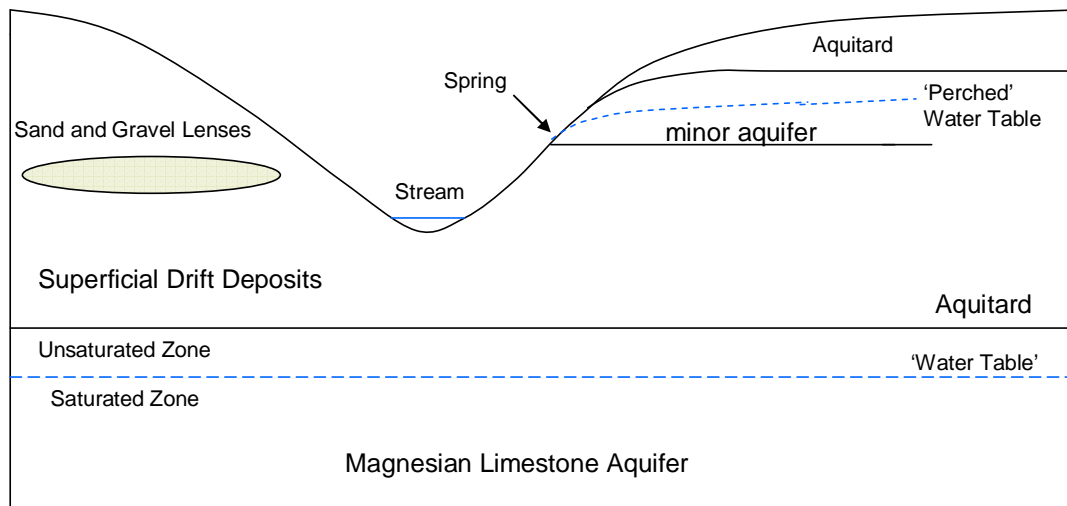
SCHEMATIC DIAGRAM OF THE 'UNCONFINED' MAGNESIAN LIMESTONE AQUIFER AND MINOR AQUIFERS OF THE SUPERFICIAL DEPOSITS.
